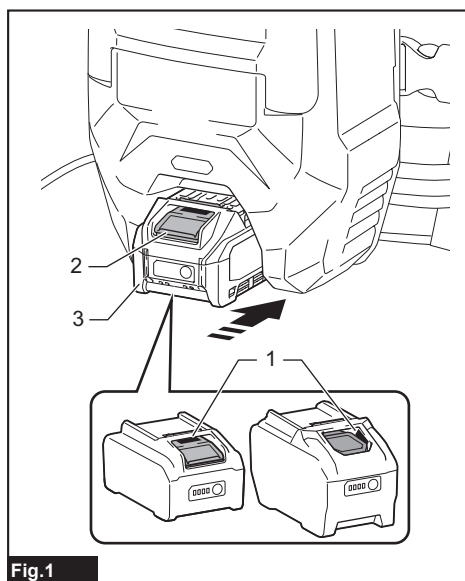
► 1. Red indicator 2. Button 3. Battery cartridge
